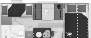
ARTICA 496 FAMILY • 5,20 x 2,15 m
